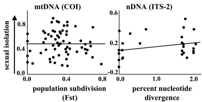
Fig. 2. The magnitude of sexual isolation observed between pairs of walking stick populations is independent of the genetic distance between pairs of populations (mtDNA: r = 0.13 , p = 0.29 ; nDNA: r = 0.29 , p = 0.10 ; Mantel tests). Sexual isolation is measured using an index where zero indicates random mating and 1 indicates complete sexual isolation. Genetic distance is calculated from DNA sequence variation at 2 independently evolving loci (mtDNA—mitochondrial locus COI; nDNA—nuclear locus ITS-2). The mtDNA data are from the 66 pairs of populations examined in Nosil et al. (2003) and the nDNA data from the 28 pairs examined in Nosil et al. (2002). The lines are least-squares regression lines, whereas significance testing was conducted using Mantel tests due to nonindependence among data points.
